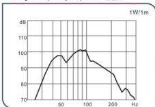
Drawing of frequency response: 頻響圖:
