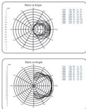
SPL dispersion illustration
